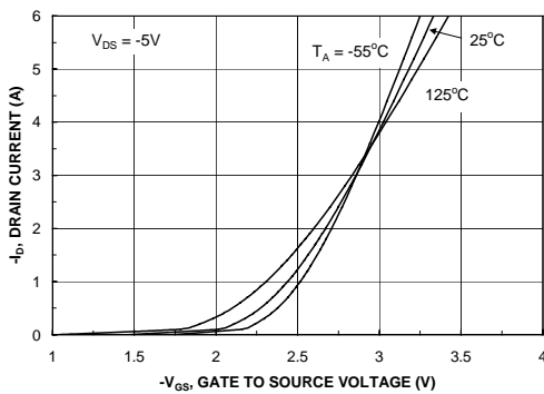
Figure 5. Transfer Characteristics.
